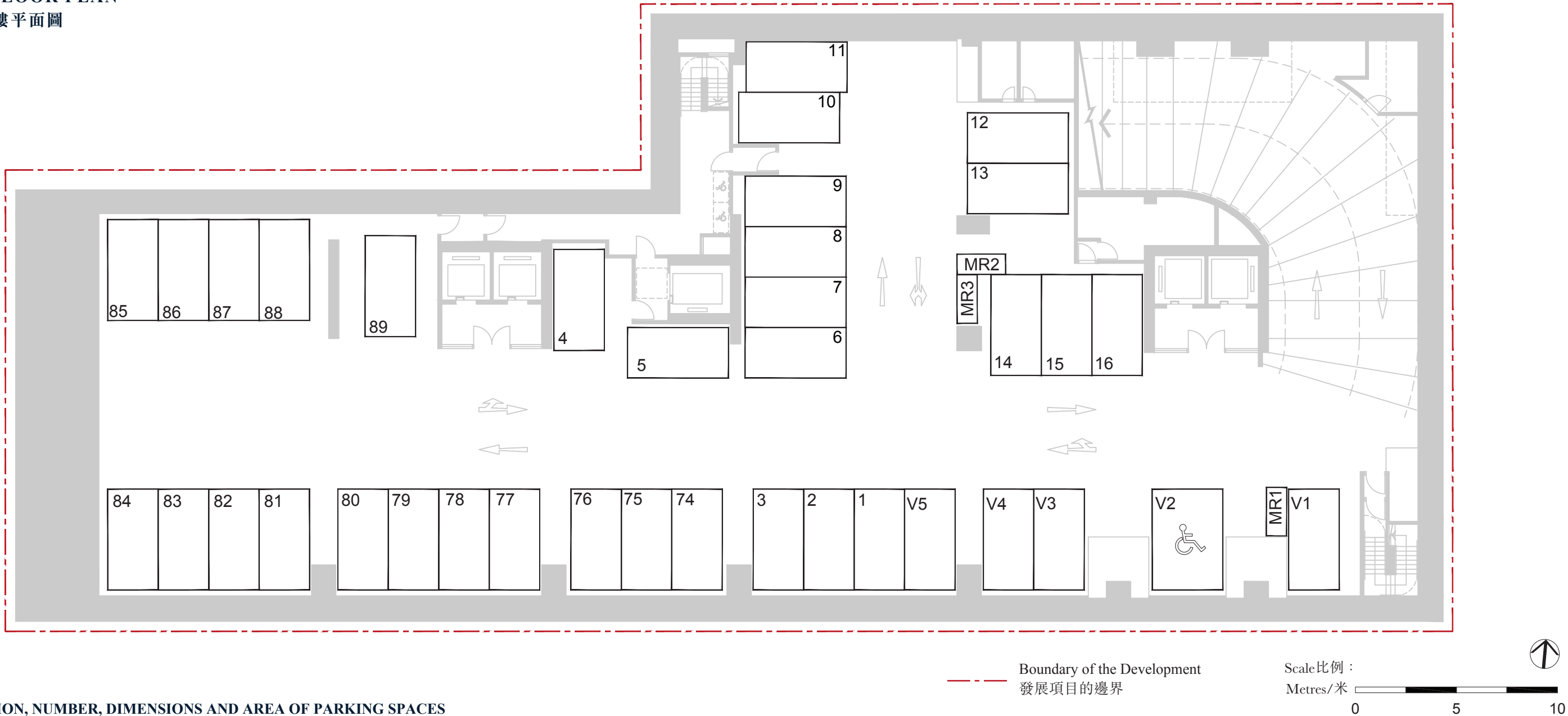
LOCATION, NUMBER, DIMENSIONS AND AREA OF PARKING SPACES 停車位位置、數目、尺寸及面積
